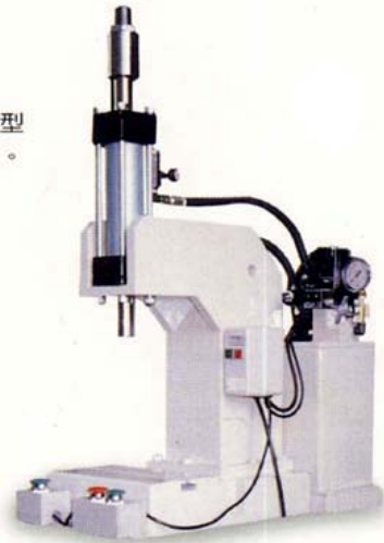
OIL PRESSURE PRESS HC-3T 油壓壓床 MAX Power : 3000 kg t/cm 2
